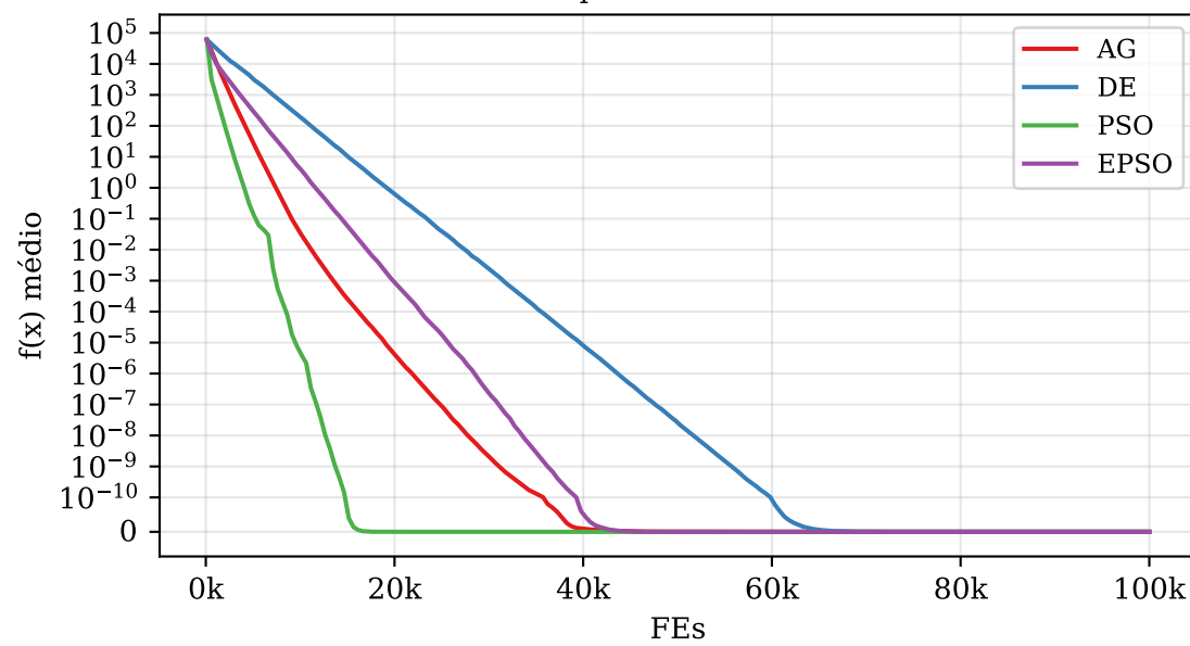
Rosenbrock — D=30
